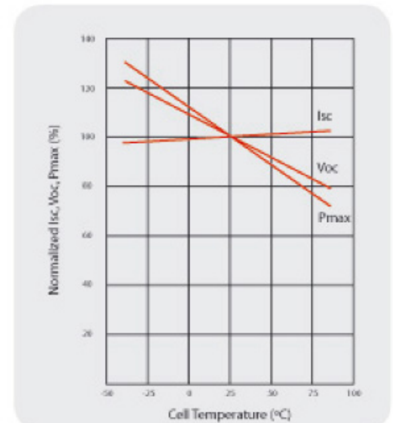
Temperature Dependence of Isc, Voc, Pmax
