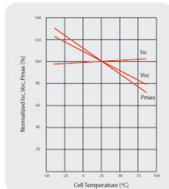
Temperature Dependence of Isc, Voc, Pmax
