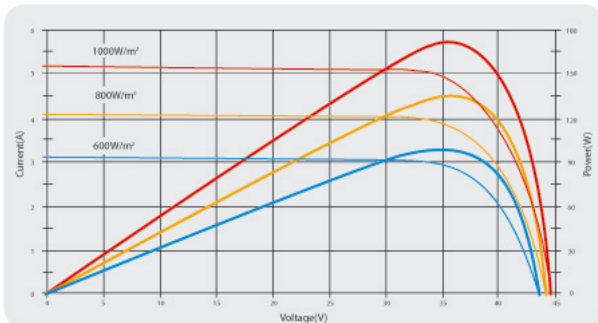
Current-Voltage & Power-Voltage Curve (175W)
